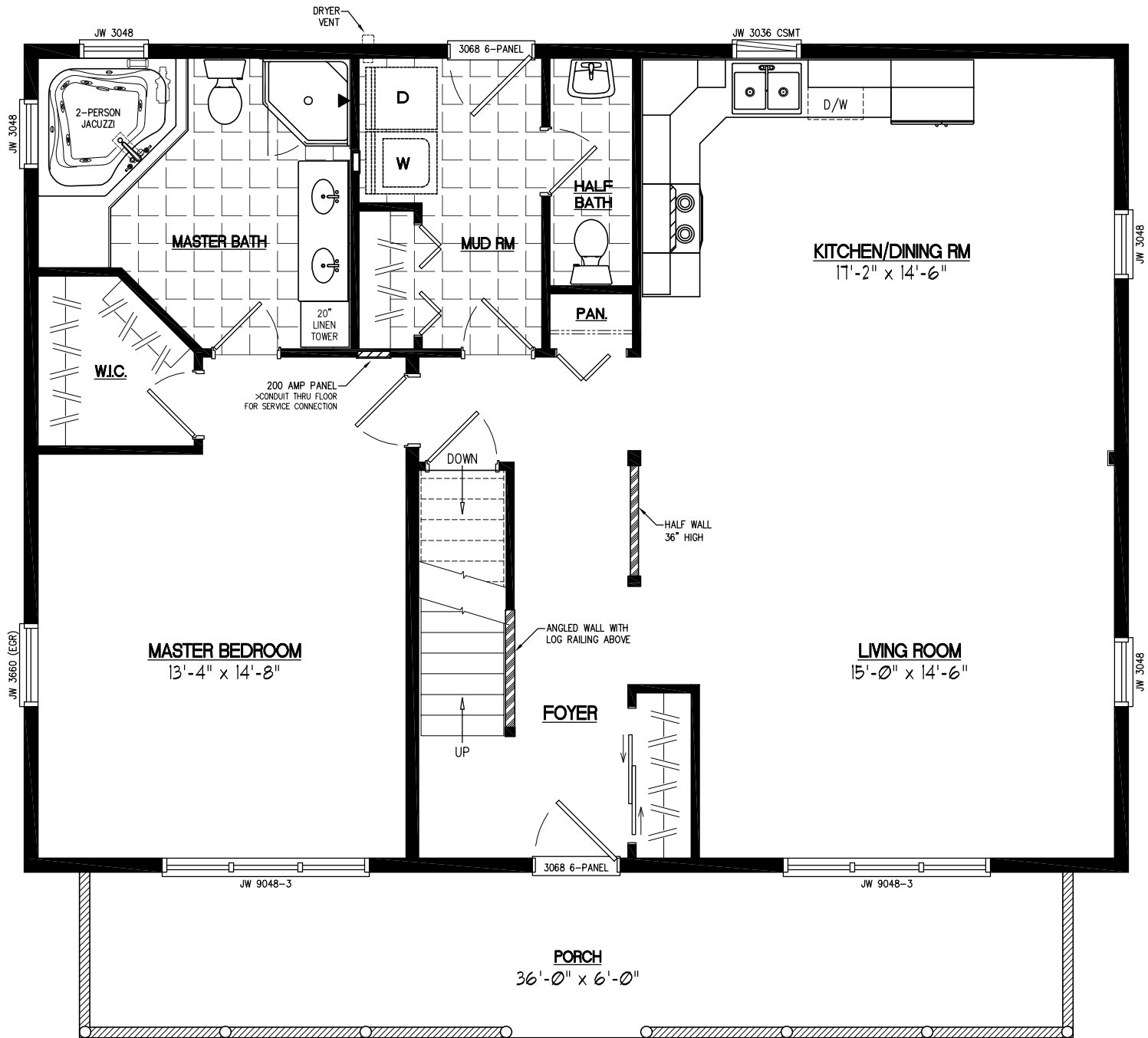
30x40 MOUNTAINEER Plan #30MR1303
