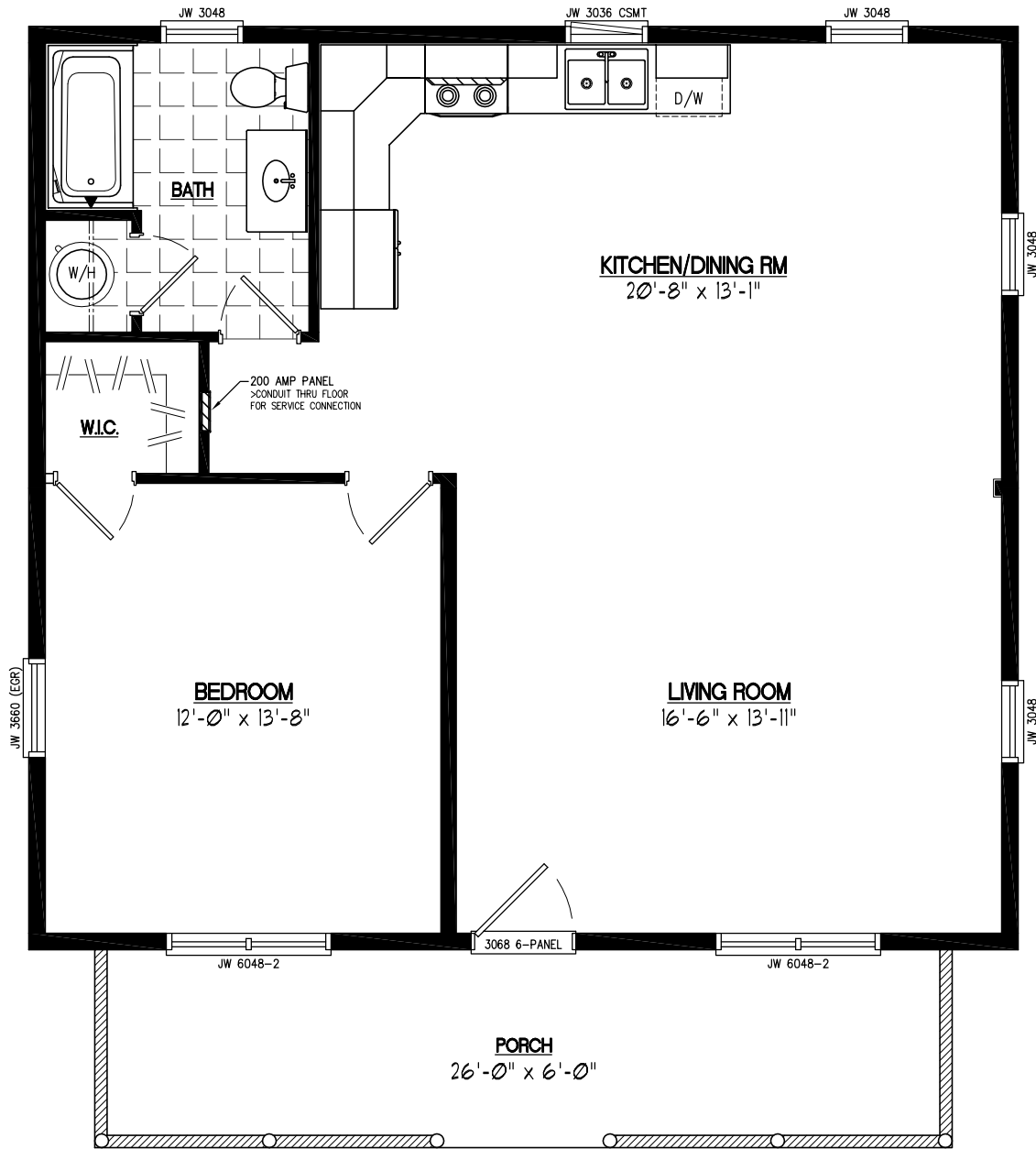
28x30 MUSKETEER Plan #28MK1501
